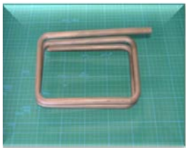
銅丸管材 12.7 × t0.8 × R 18 Copper round pipe
