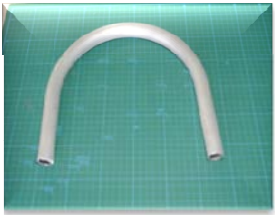
アルミ合金60系丸管材 25.0 × t1.5 × R125 Aluminum alloy(60 series) round pipe
