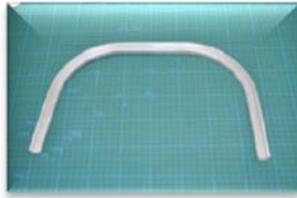
アルミ合金60系異型管材 C21 \times 12 \times t1.0 \times Ri100 Aluminum alloy(60 series)
