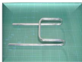
STKM丸管材 12.0 × t1.6 × R25 STKM round pipe
