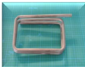
銅丸管材 12.7 × t0.7 × R 18 Copper round pipe
