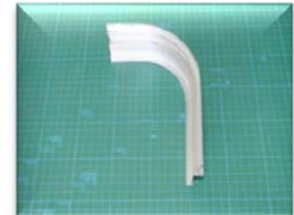
アルミ合金60系異型材 □58 × 12 × t1.0 × Ri60 Aluminum alloy(60 series)
