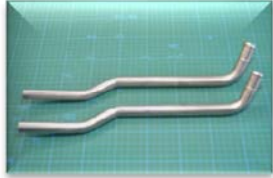
SUS304丸管材 17.0 × t0.8 × R18 SUS304 round pipe
