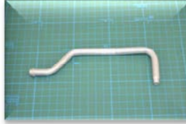
アルミ合金丸管材 9.53 \times t1.0 \times R10 Aluminum alloy(60 series) round pipe
